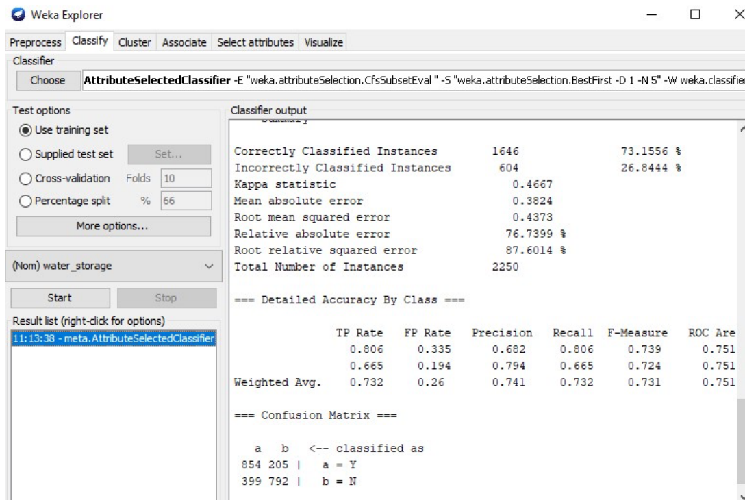
Figure B. Performance Evaluation Matrix in WEKA.
